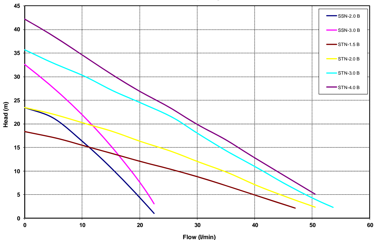
Brass Universal Head Pump Range - Performance Curves
